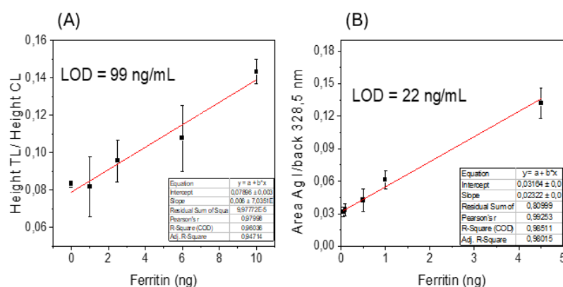
Ferritin calibration curves obtained via LFIA (A) and LIBS (B).
