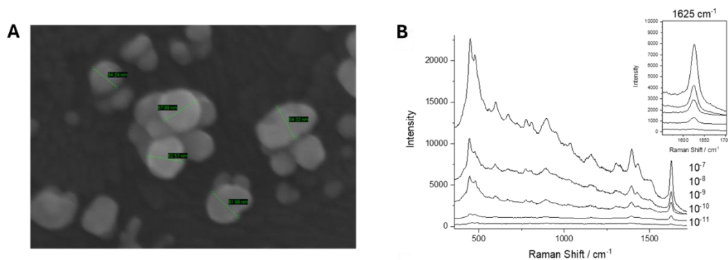
Figure 1. (A) SEM image of Mel@Ag nanostructures showing nanoparticle organization and dimer formation. (B) SERS spectra of L-Dopa at decreasing concentrations, demonstrating detection down to 10 -11 M.
